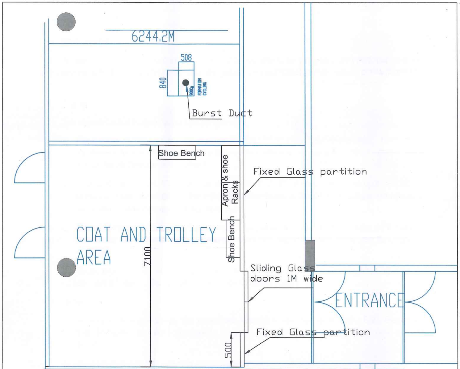
Glass Partition Layout
